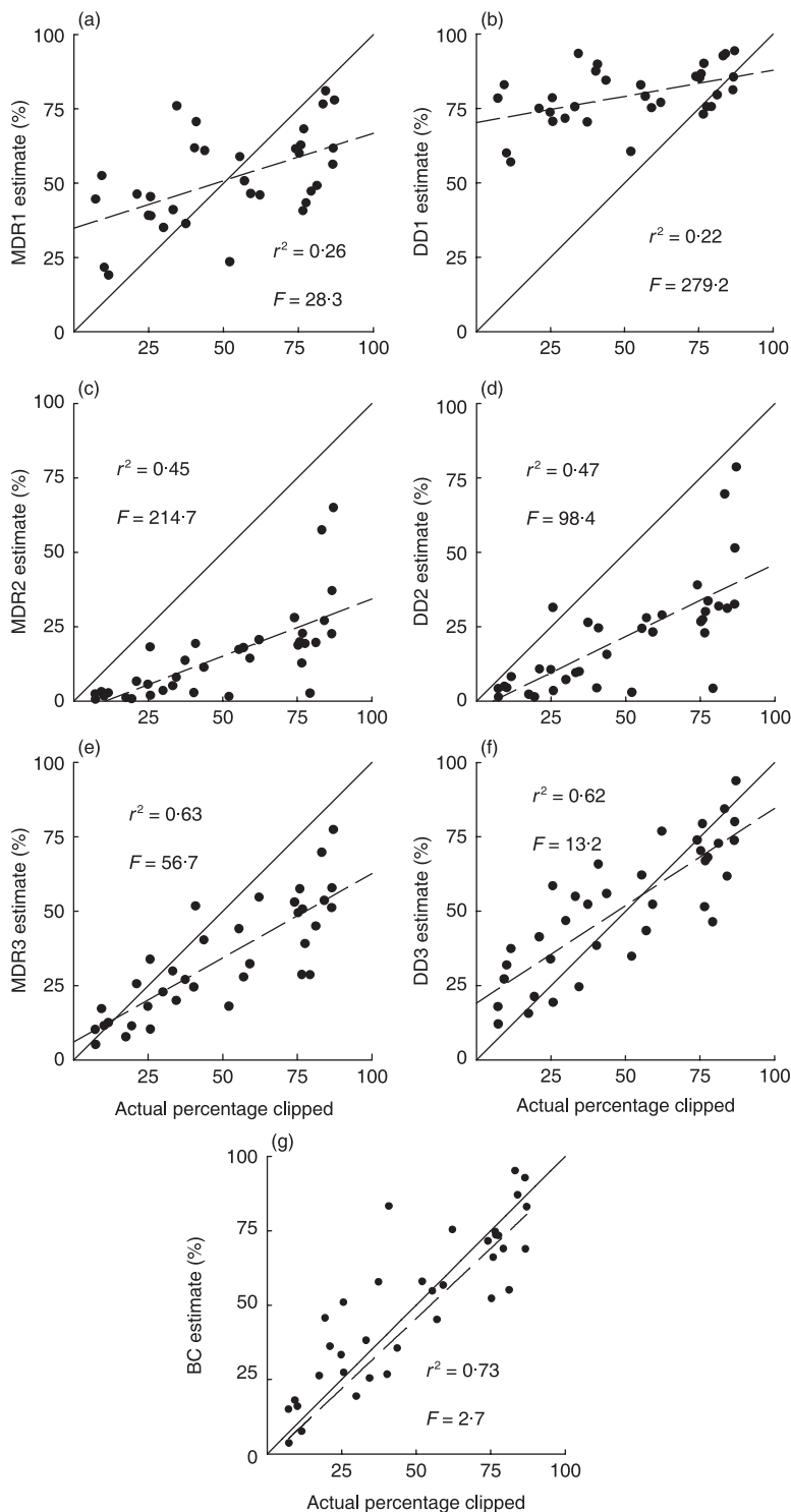
Fig. 2. Results of regressing actual percentage clipped of S. bebbiana stem current annual growth against estimates by seven methods: two shoot-level methods, (a) the mass-diameter regression (MDR) method and (b) the diameter difference (DD) method, scaled by taking a simple average; the MDR method (c) and the DD method (d) scaled by multiplying by the proportion of browsed shoots; the MDR method (e) and the DD method (f) scaled by multiplying by the proportion of shoot mass browsed; and (g) the biomass comparison (BC) method. A perfect model would conform to the solid 1:1 line; dashed lines indicate a linear least-squares fit to the data. F -values indicate the magnitude of deviation of the dashed line from the 1:1 line.
