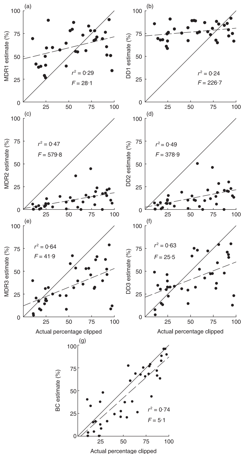
Fig. 3. Results of regressing actual percentage clipped of S. geeyeriana stem current annual growth against estimates by seven methods: two shoot-level methods, (a) the mass-diameter regression (MDR) method and (b) the diameter difference (DD) method, scaled by taking a simple average; the MDR method (c) and the DD method (d) scaled by multiplying by the proportion of browsed shoots; the MDR method (e) and the DD method (f) scaled by multiplying by the proportion of shoot mass browsed; and (g) the biomass comparison (BC) method. A perfect model would conform to the solid 1:1 line; dashed lines indicate a linear least-squares fit to the data. F -values indicate the magnitude of deviation of the dashed line of the 1:1 line.
