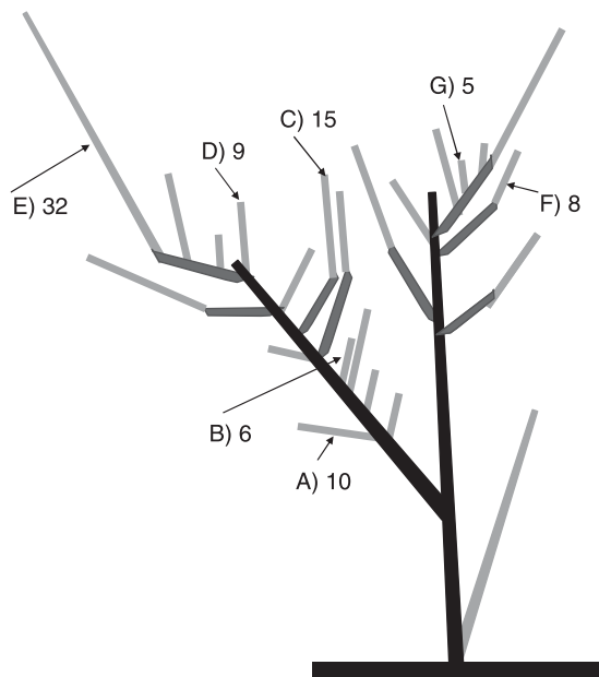
Fig. 1. Diagram illustrating shoot sampling protocol for a stem. Letters indicate the order of measurements; numbers indicate lengths in centimetres. To represent adequately the shoot size distribution in this example, we chose a sampling ratio of 3, which means we recorded measurements on every third shoot encountered as we worked apically from the base of the stem, accommodating side branches by sampling the lowest branches first. Here, seven measurements were made, with two shoots apical of the last shoot sampled. The count of shoots was then calculated as 7 \times 3 + 2 = 23 . If four of the seven measured shoots were browsed, along with the two apical of the last shoot sampled, then the count of browsed shoots is estimated as 4 \times 3 + 2 = 14 , and the count of un browsed shoots as 3 \times 3 + 0 = 9 .
