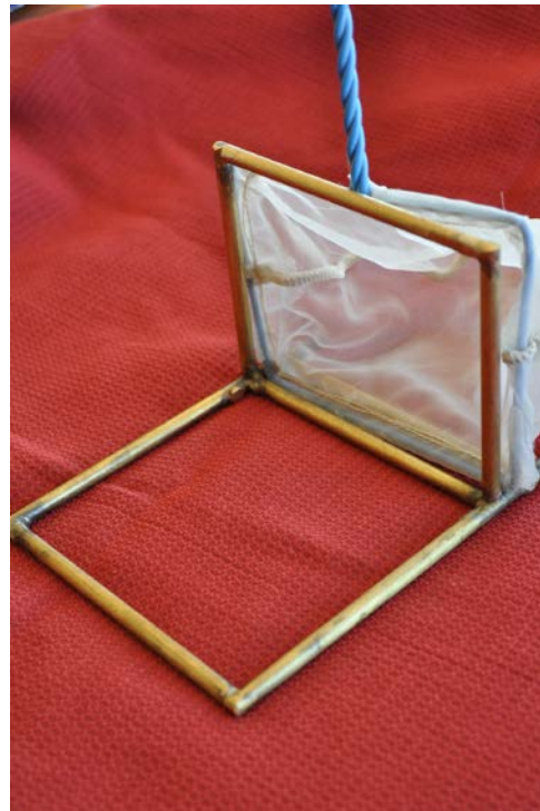
Figure 22. A) 10 cm X 20 cm brass quadrat, B) 10 cm X 20 cm brass quadrat with 10 cm X 20 cm, 250 µm mesh dipnet.
