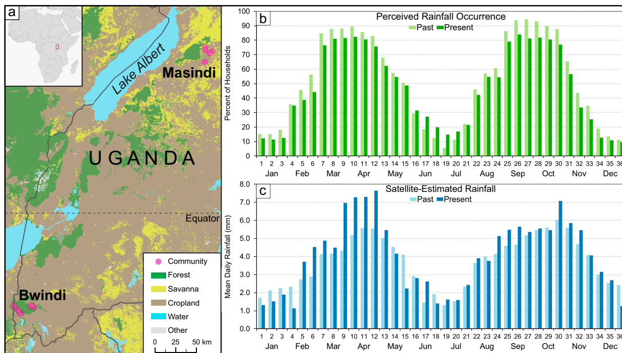
FIG. 1. Intra-annual seasonal rainfall patterns in western Uganda. (a) Study region in the climatic transition zone of eastern and central equatorial Africa, land cover (Friedl et al. 2010), and locations of study communities in the northern and southern sites. (b) Percentage of farmer respondents ( n = 614 ) observing rainfall presence (1/0) in 36 dekadal periods (January–December), reported through surveys, and corresponding to recent (last few years) and past periods (10–20 years). (c) Mean total rainfall (mm) averaged across Masindi and Bwindi sites in 36 dekadal periods (January–December); data represent mean values from two validated satellite-based rainfall products in recent (2014–18) and past periods (1998–2008) (Funk et al. 2015; Maidment et al. 2017). See Fig. S1 in the online supplemental material for higher-resolution longitudinal comparisons of rainfall and temperature.
