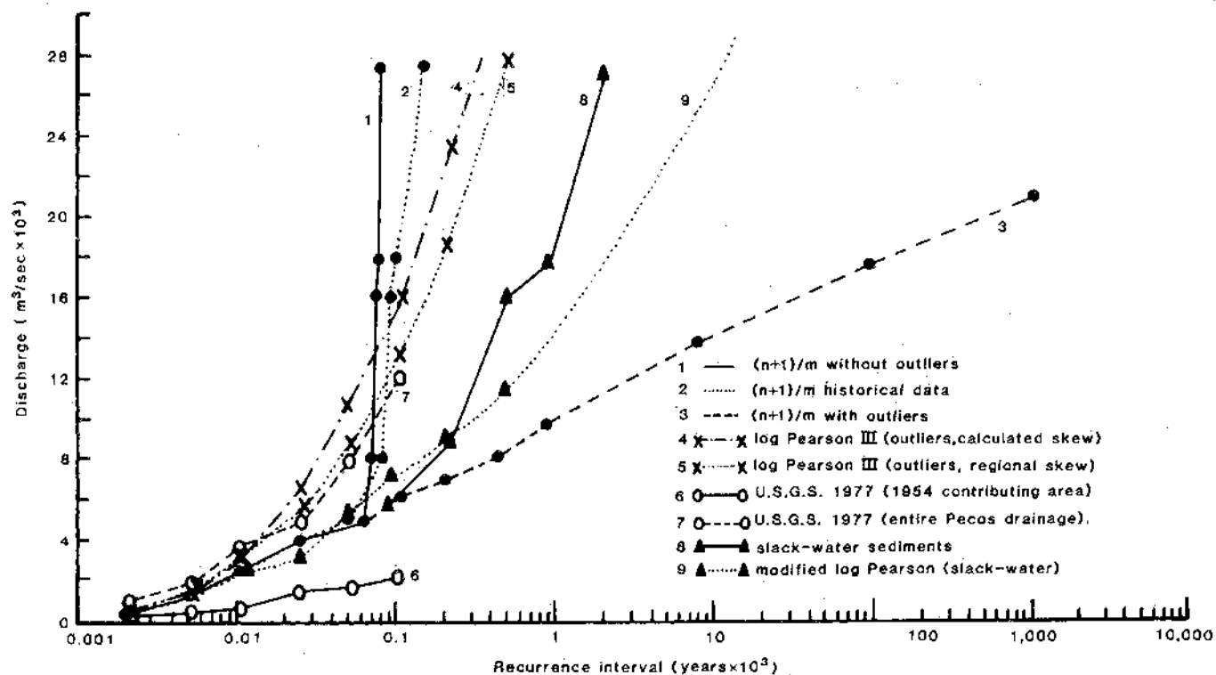
Fig. 8. Comparison of various techniques for estimating flood frequency in the lower Pecos River region near Langtry. Curves 1 to 7 illustrate techniques using historical data while curves 8 and 9 illustrate modifications using slack-water sediment data over the past 10,000 years. Data for these curves are summarized in Table 3.
