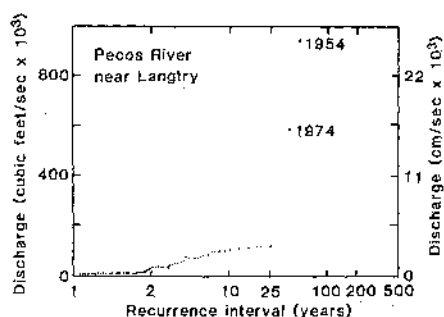
Fig. 5. Flood frequency plot for the Pecos River near Langtry, Texas, for the period 1900 to 1980. Note that the 1954 and 1974 floods occur as extreme outliers. Data from International Boundary and Water Commission (24).
