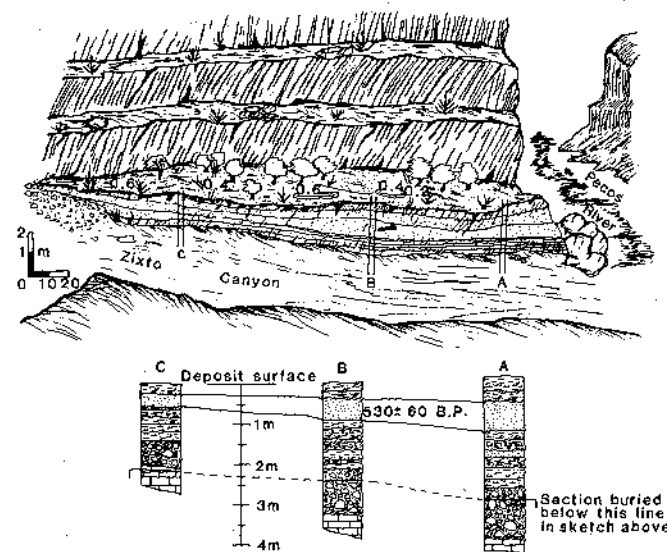
Fig. 4. Schematic drawing of the slack-water deposit in Zixto Canyon. Contours are at 0.2-m intervals on the deposit surface. Note that some units pinch out up the tributary canyon.
